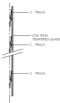
STYLE 21 NON-MAGNETIC
