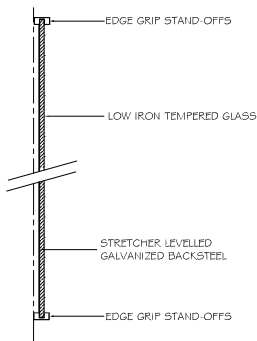
STYLE 20 MAGNETIC
